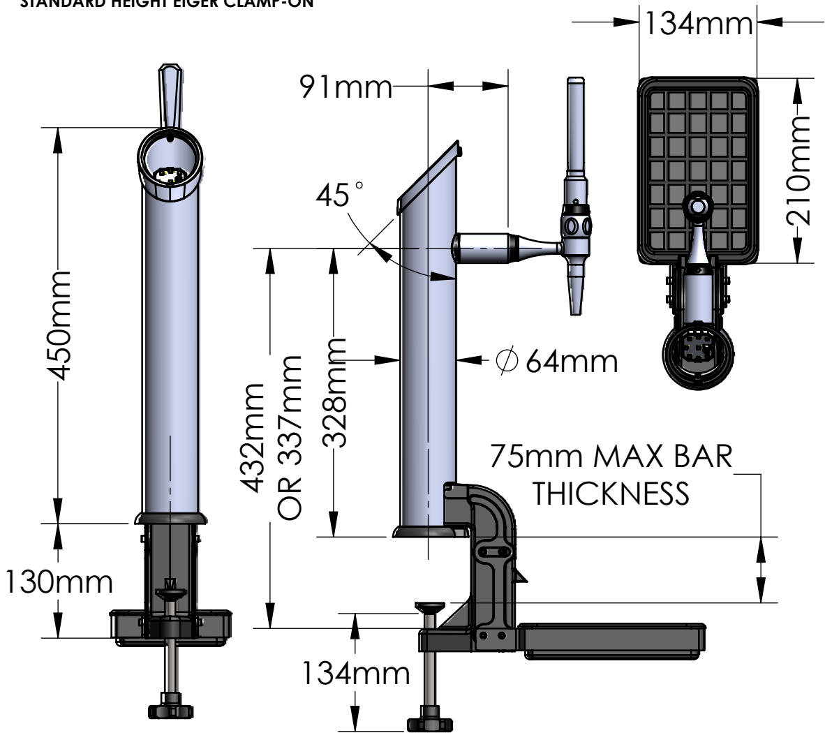
STANDARD HEIGHT EIGER CLAMP-ON
