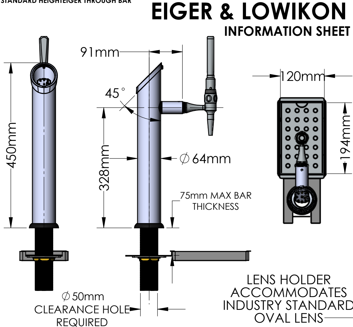
STANDARD HEIGHT EIGER THROUGH BAR
